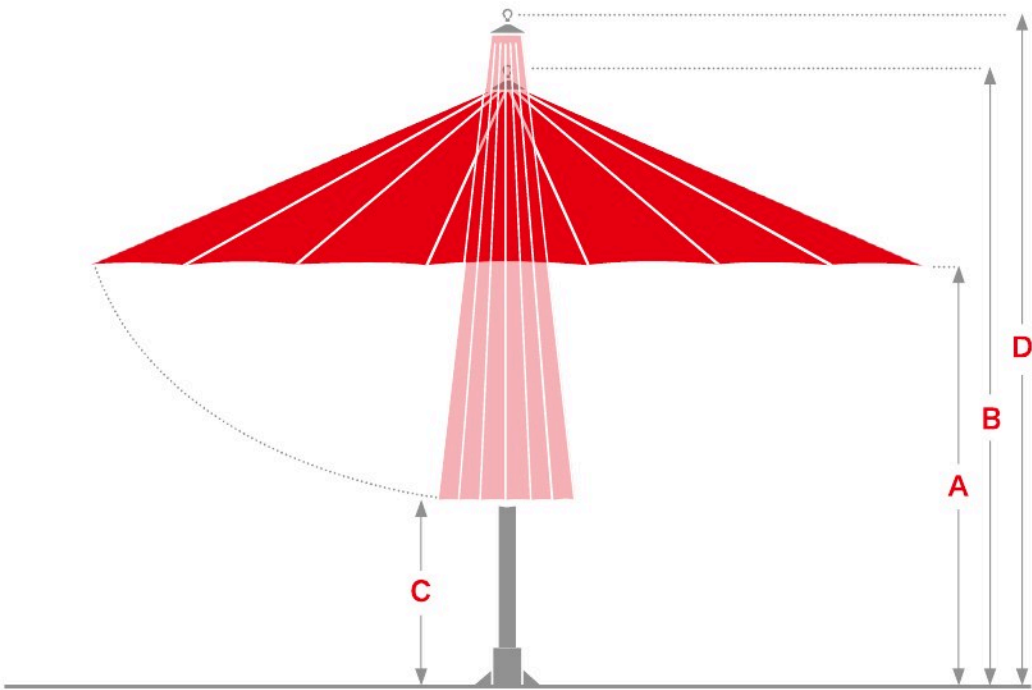
Diagram: Ø 15 m A: Open edge height 350 cm B: Open total height 640 cm C: Closed edge height 196 cm D: Closed total height 985 cm
